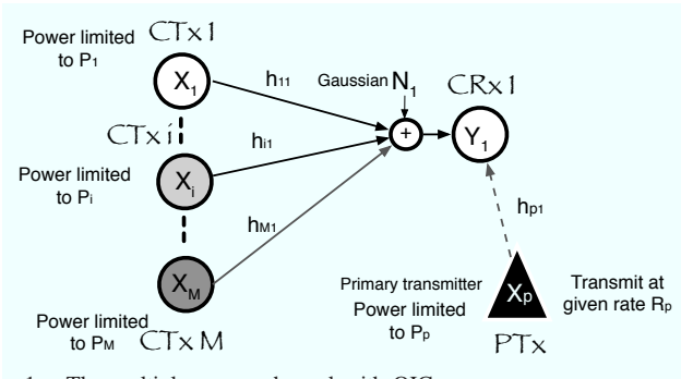
Fig. 1. The multiple access channel with OIC.
