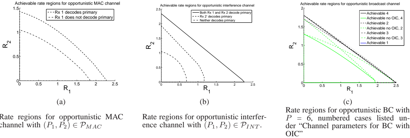
Fig. 4. Impact of opportunistic interference cancellation.
